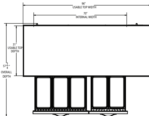
PLAN VIEW
