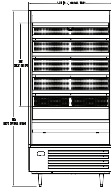
ELEVATION VIEW
