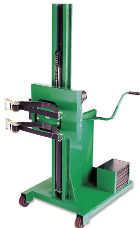
Manual Strap Connection - Counterweighted
