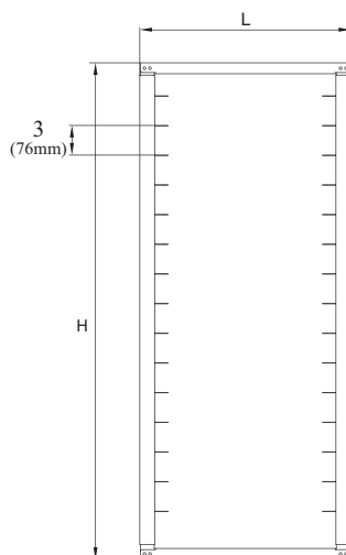
TSP-2250-T FRONT VIEW
