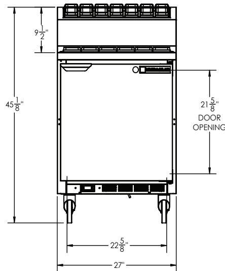
ELEVATION VIEW
