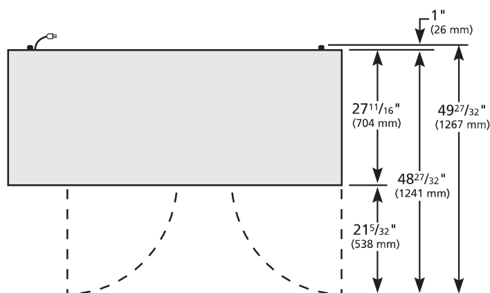
PLAN VIEW
