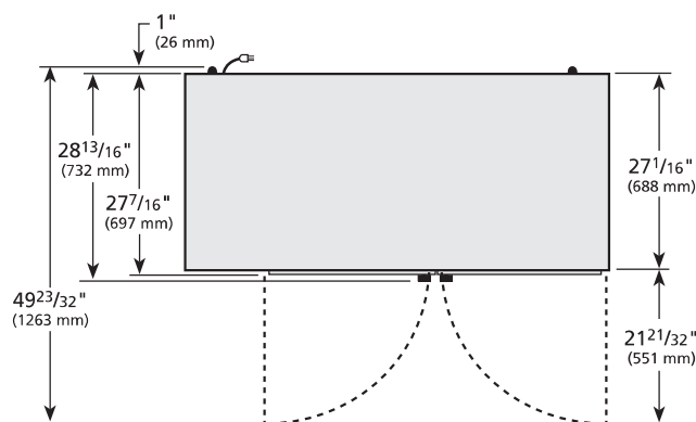
PLAN VIEW
