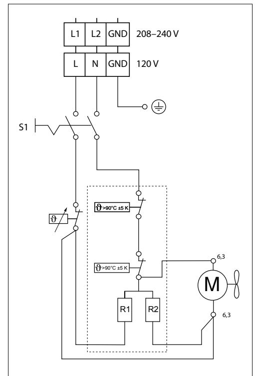
Wiring diagram CK 150-1 Plus, CK 200-2 Plus
