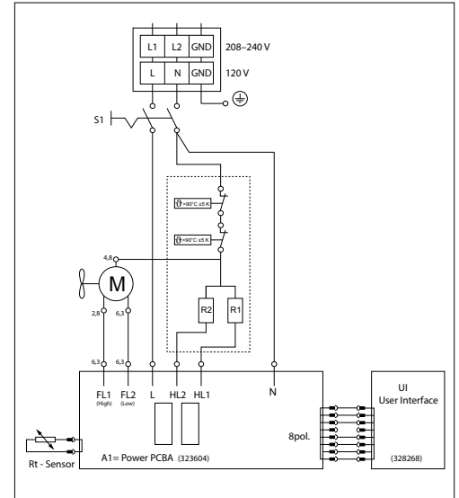
Wiring diagram CK 150-1 Plus, CK 200-2 Plus
