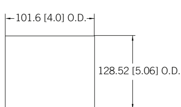
SHORT SLEEVE
