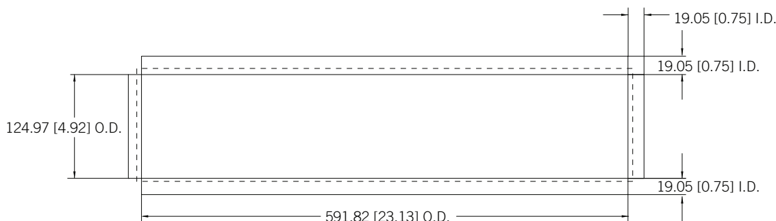
SLEEVE
