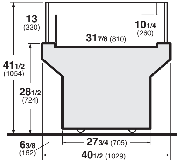
Cross Section
