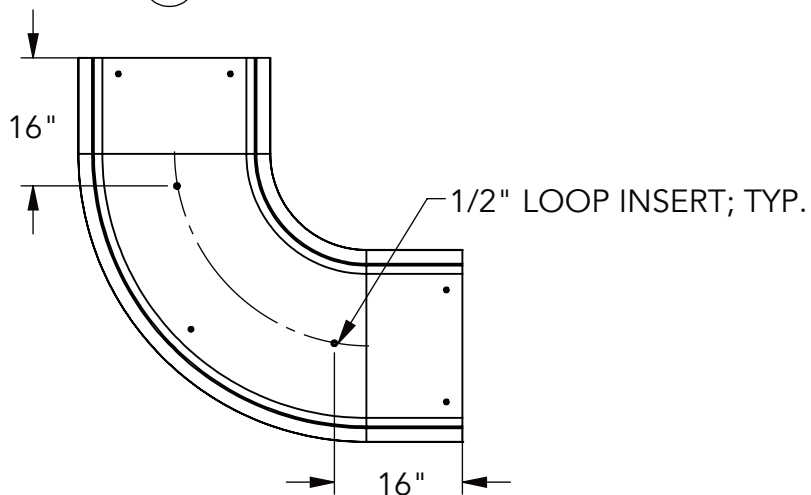
③ BOTTOM VIEW
