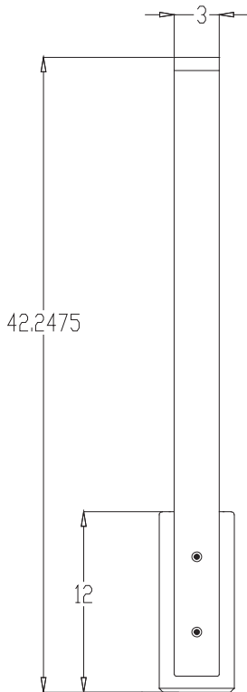
ELEVATION VIEW
