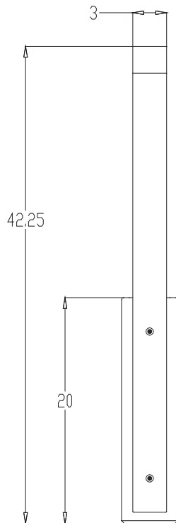
ELEVATION VIEW
