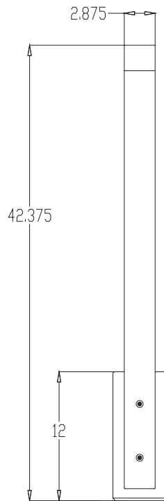
ELEVATION VIEW
