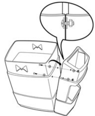
Hardware for Side Pods #8178088009 Includes: 8 washers, 4 screws, 4 nuts and instruction sheet. Need: 2 sets for 2 side pods
