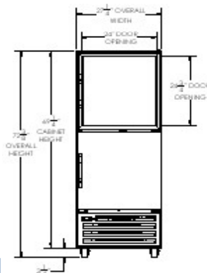
ELEVATION VIEW
