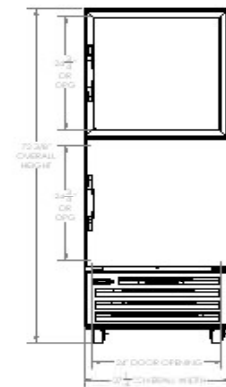
ELEVATION VIEW
