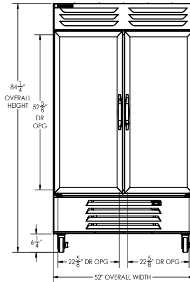
ELEVATION VIEW
