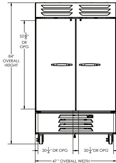
ELEVATION VIEW
