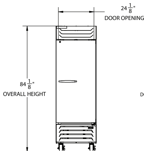
ELEVATION VIEW
