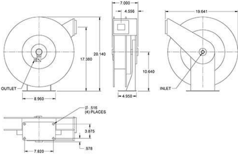
7000 SERIES OXP SW DIMENSIONAL DRAWING
