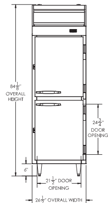
ELEVATION VIEW
