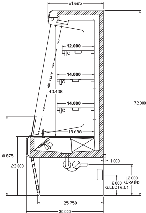
CROSS SECTION
