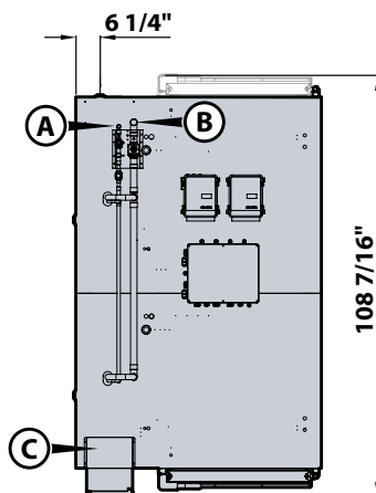
DRAIN POSITION
