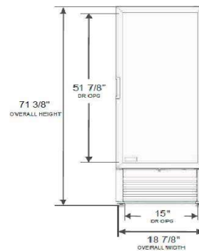
ELEVATION VIEW
