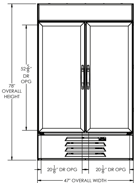
ELEVATION VIEW
