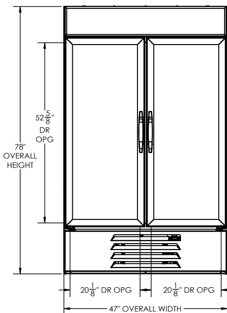
ELEVATION VIEW
