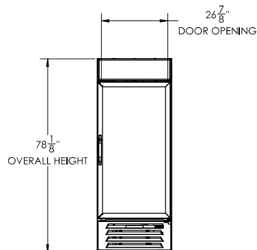
ELEVATION VIEW
