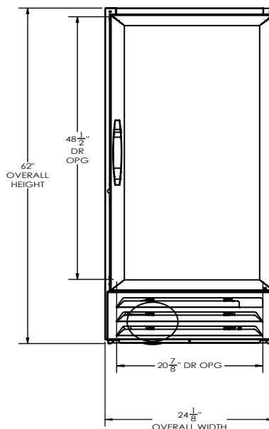
ELEVATION VIEW
