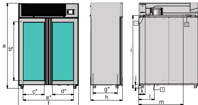
200kg Capacity Model MATC200TF
