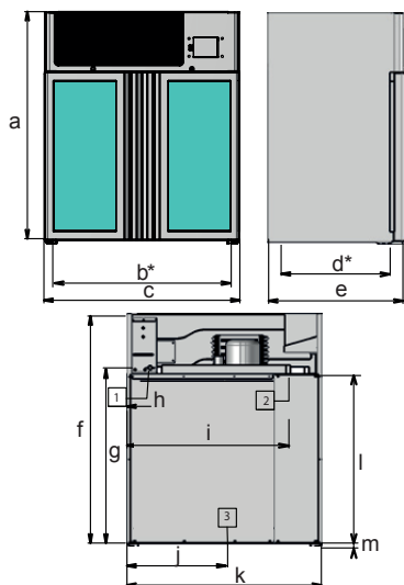
60kg Capacity Model MATC060TF
