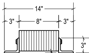
FRONT VIEW 3/8" GAP
