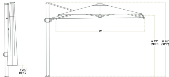
Pink/Crank Cantilever Umbrella with Lights - 10' x 10'
