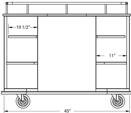
Model 8715
