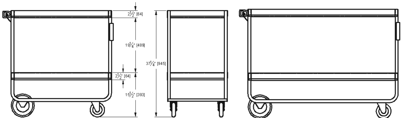
Model 727
