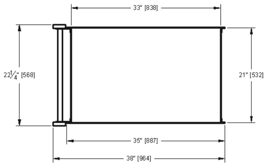
Model 727
