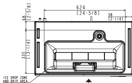
REMOTE AIR-COOLED
