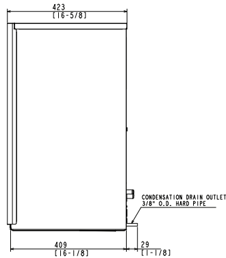
REMOTE AIR-COOLED
