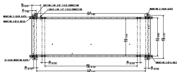
SRK-15J(3) REMOTE CONDENSER
