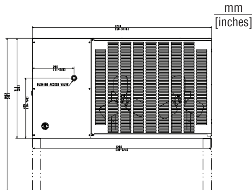
SRK-15J(3) REMOTE CONDENSER
