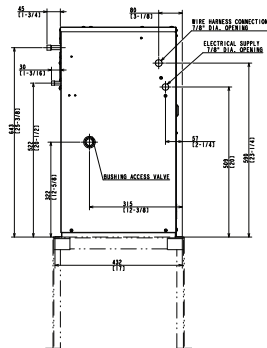
SRK-15J(3) REMOTE CONDENSER
