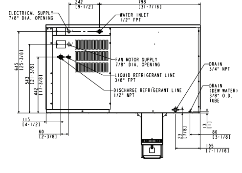
REMOTE AIR-COOLED
