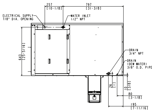
AIR-COOLED
