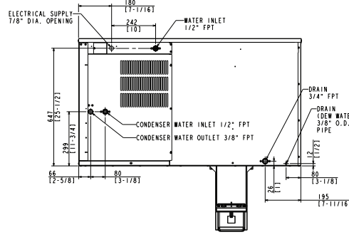
WATER-COOLED
