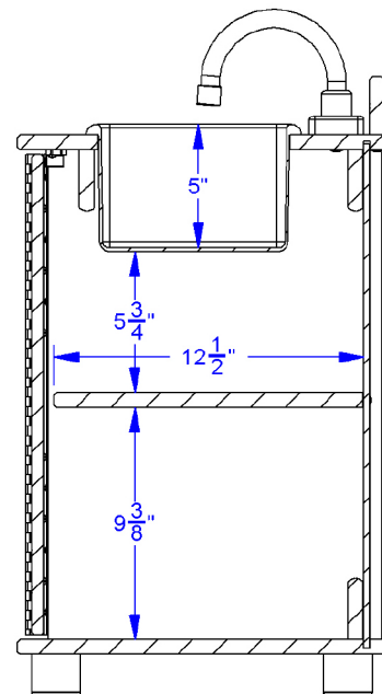
SECTION VIEW
