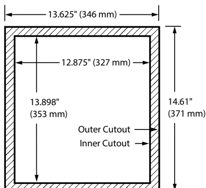
Cutout Dimensions for Flush Mount
