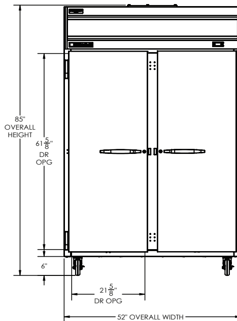
ELEVATION VIEW
