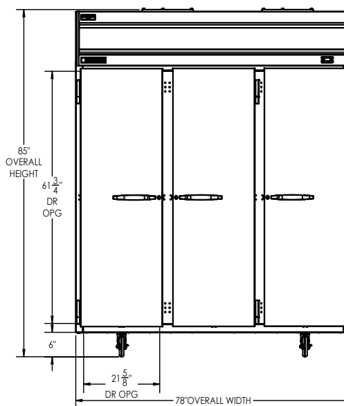
ELEVATION VIEW
