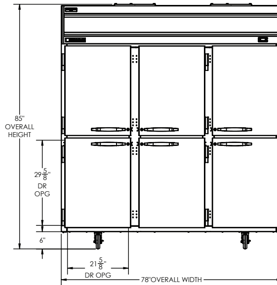
ELEVATION VIEW
