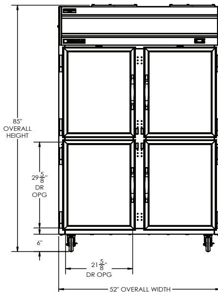
ELEVATION VIEW
