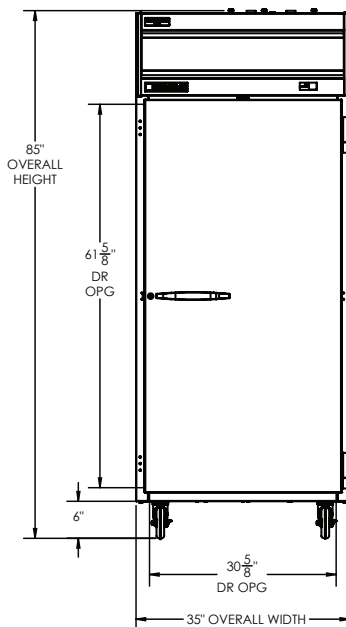
ELEVATION VIEW
