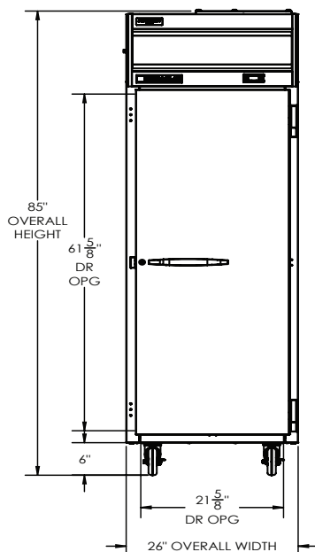
ELEVATION VIEW
