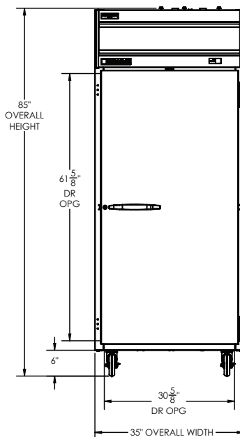
ELEVATION VIEW
