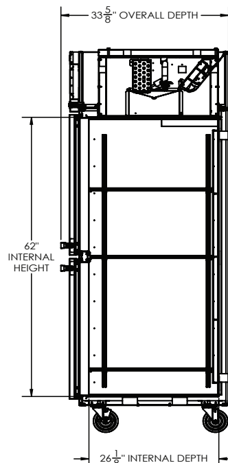
SIDE VIEW
