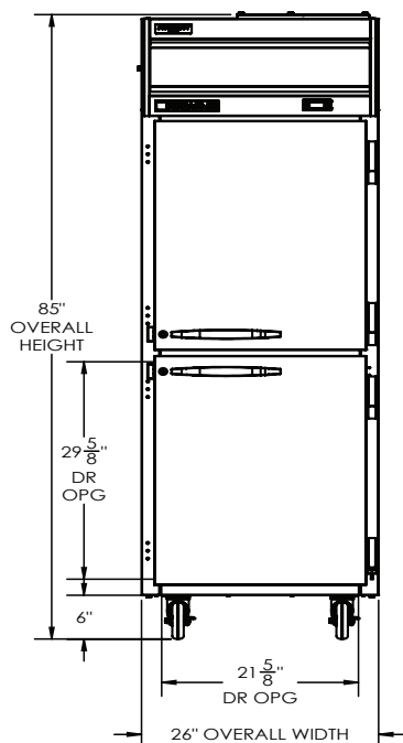
ELEVATION VIEW
