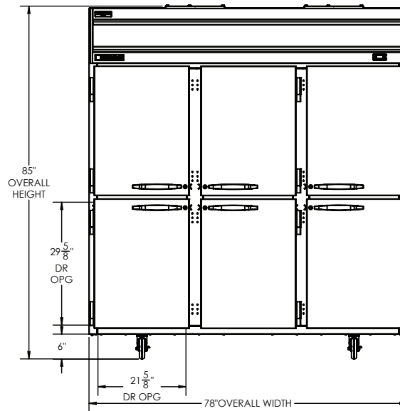
ELEVATION VIEW
