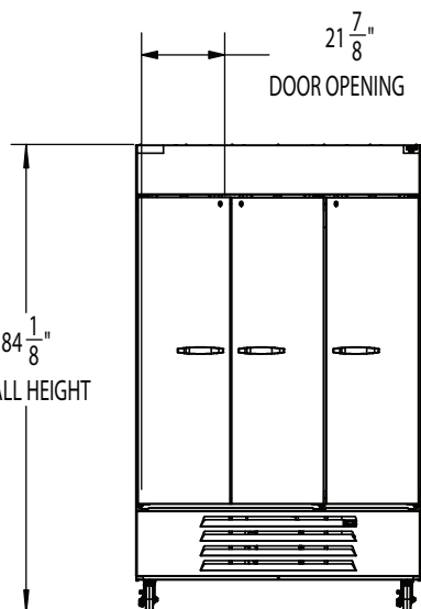
ELEVATION VIEW
