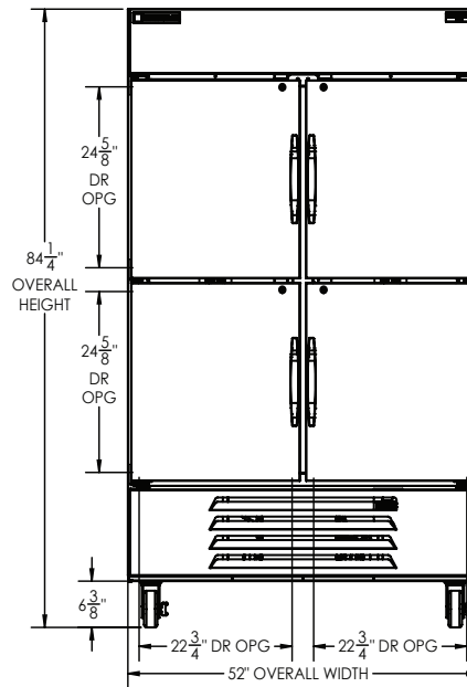
ELEVATION VIEW
